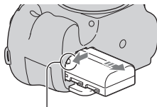
Lock lever
