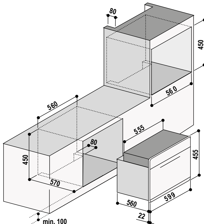
Joonis A – mudel VIRTUS COMBI STEAM MW TFT BL/6045 - PRF0191769
