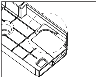
Right bracket front slot
