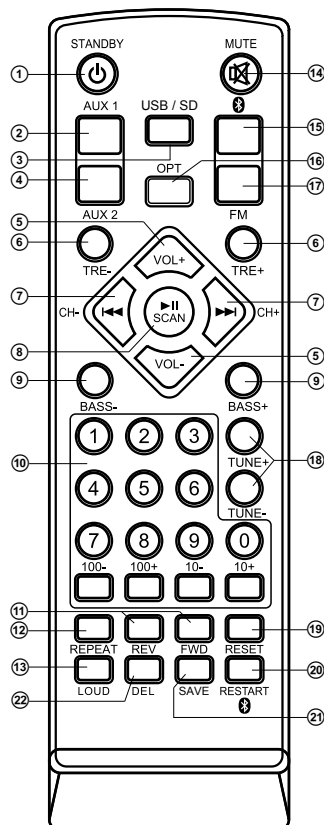
Fig. 3. Remote control
