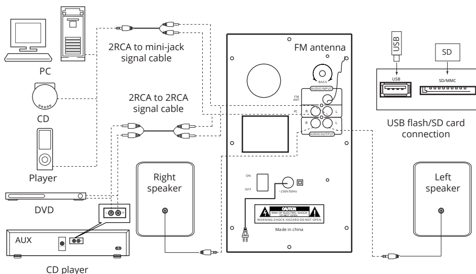
Fig. 4. Connection diagram
