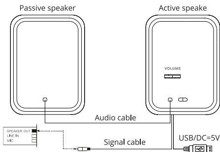
Fig. 2. Connection diagram
