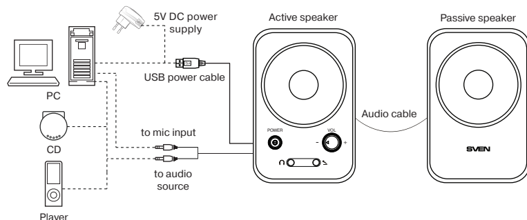
Fig. 2. Connection diagram
