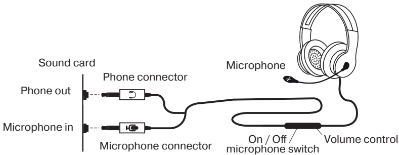
Fig. 1. Connection diagram
