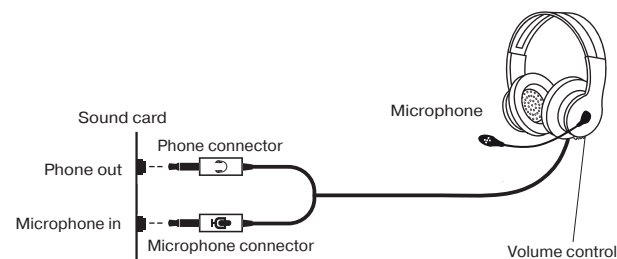
Fig. 1. Connection diagram
